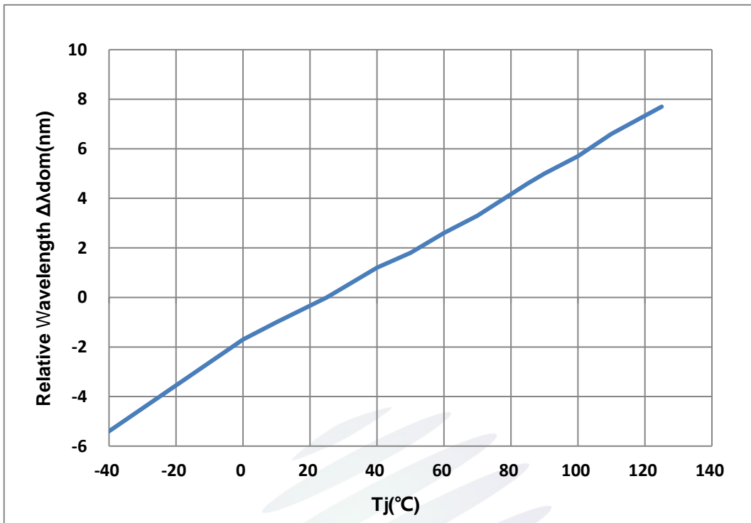
Fig. 1-13 Chromaticity Coordinate Vs Solder Temperature 波长与结温特性曲线
