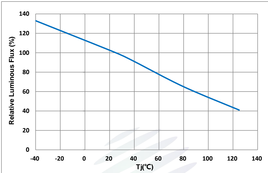
Fig. 1-9 Junction Temperature Vs Relative Intensity 结温与相对光通量特性曲线
