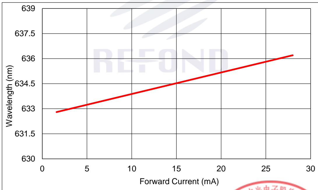
Fig.1-11 Forward Current Vs Dominate Wavelength (Ta=25°C) 正向电流与主波长关系曲线 (红光)
