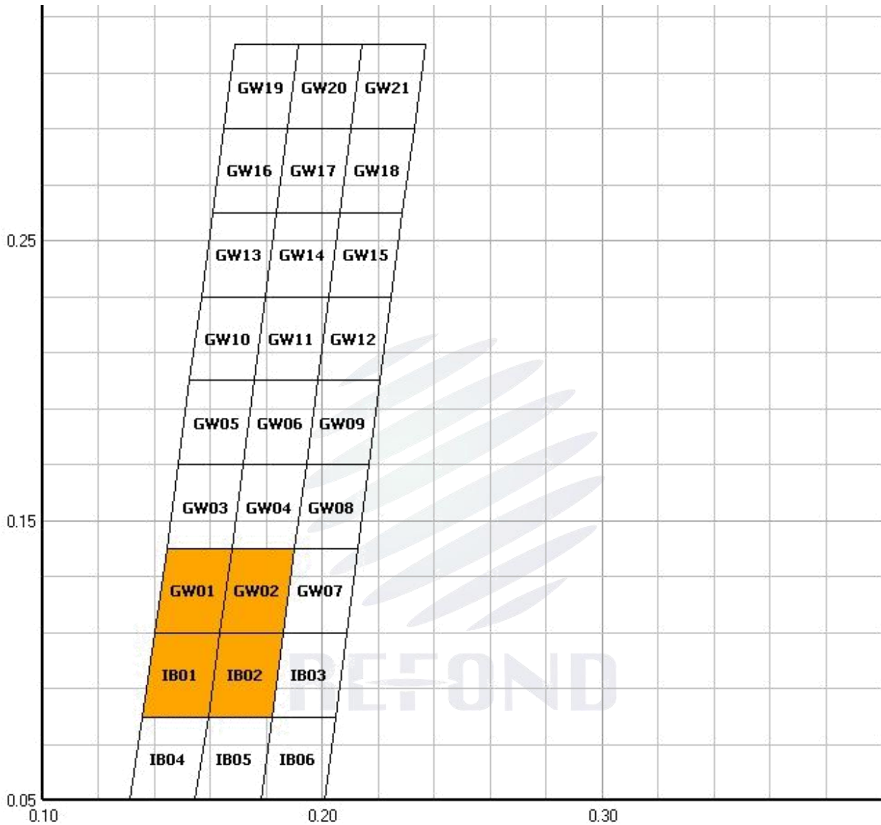
Fig. 1-6 The C.I.E Chromaticity Diagram CIE色度图
