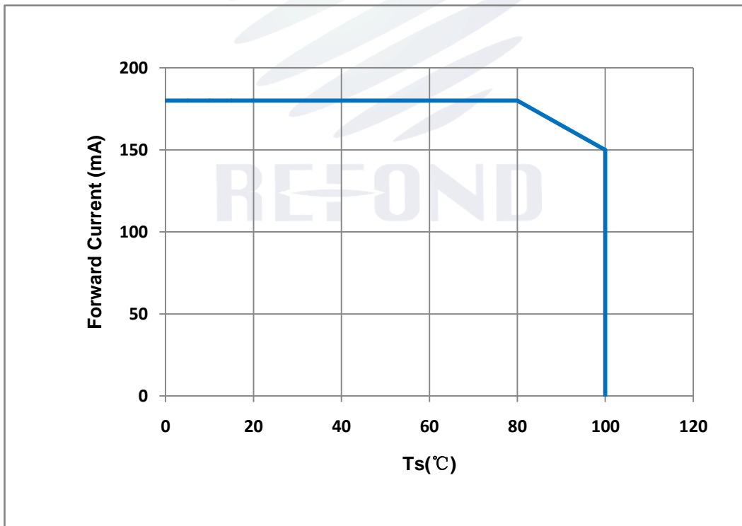
Fig 1-12 Solder Temperature Vs Forward Current 管脚温度与正向电流特性曲线
