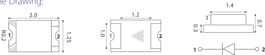
Package Outline Drawing:
