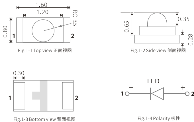
Package Outline Drawing:
