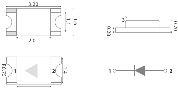
Package Outline Drawing:
