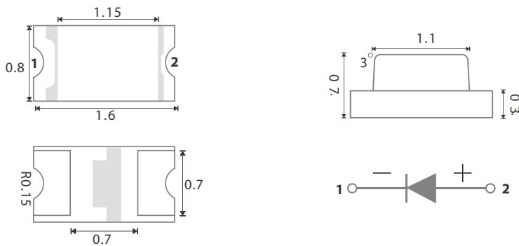
Package Outline Drawing:
