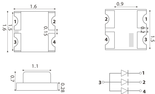
Package Outline Drawing:
